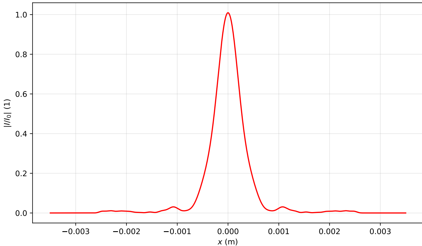
Intensity profile I(x, y = 0, z = 3.582)/I_0 , P_{in}=2.0P_{cr} , artificial time
